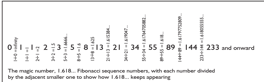
Figure 9-1: A graph showing Fibonacci ratios of 1.618...
