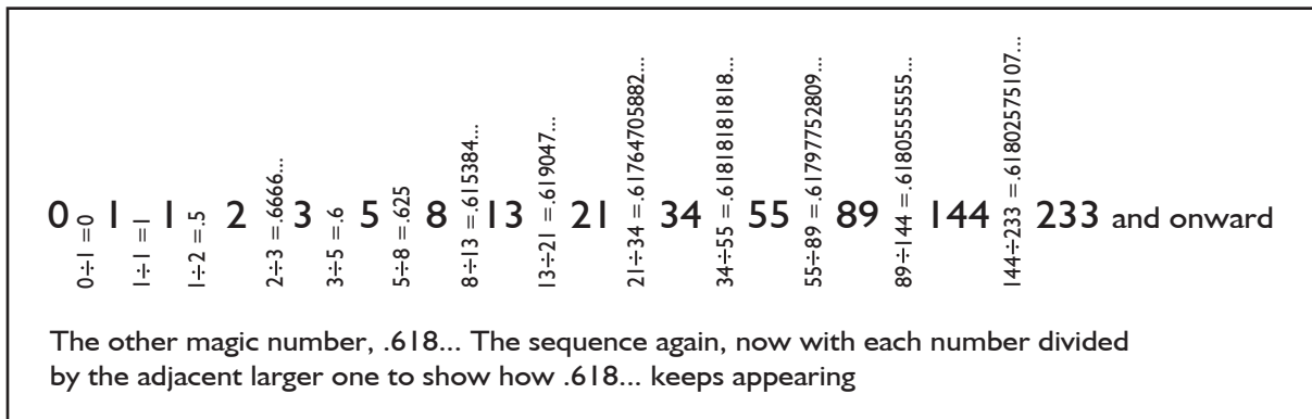
Figure 9-2: A graph showing Fibonacci ratios of .618...
